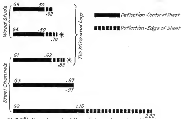
Effect of Tie Wire and Lap in Reducing Deflection of Lath under Trowel. Showing tie wire not needed on wood studs.
